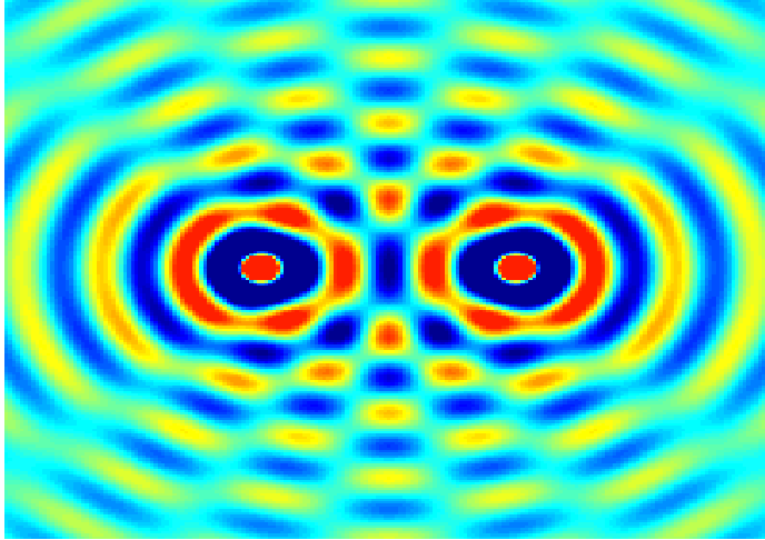
Figure 7. Interference of waves coming from two point sources.
