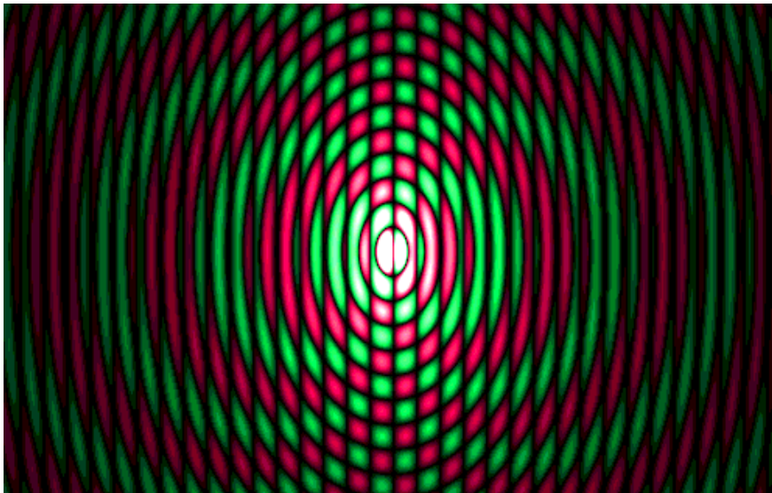
Figure 10. The electron is a spherical standing wave system.
