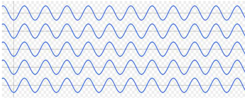
Figure 6. In-phase-waves (re-established meridian field)
