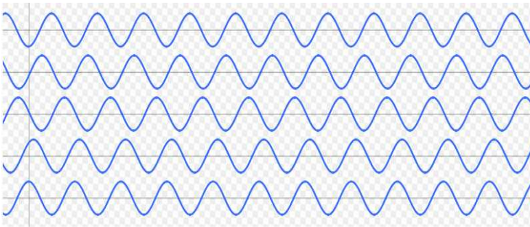
Figure 5. Out-of-phase waves distorting a meridian field (wave system)
