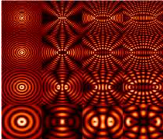
Figure 2. Waves create interference patterns. Interference patterns convey information, for the shape of the medium in which the two or more waves are moving together changes as a result of their interaction. Over time, the waves move apart from their centers (right column), but areas of destructive interference remain stable. The pattern is like a signature or key which causes the new interference pattern (wave) to resonate at a very distinct permittivity or dielectric constant. Thus it will couple with certain other structures (retina) if it matches with those wave systems. Waves do not have to be of the same amplitude in order to match. They could match on a different levels (octaves).
