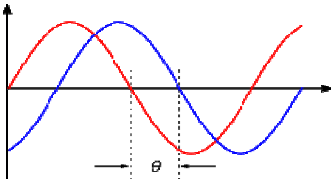
Figure 8. Phase shift. When two matching waves entangle, the new coupled oscillating wave system will have a slight phase shift. This is information.
